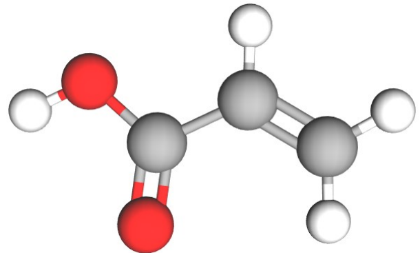
*Image depicts Acrylic Acid*
